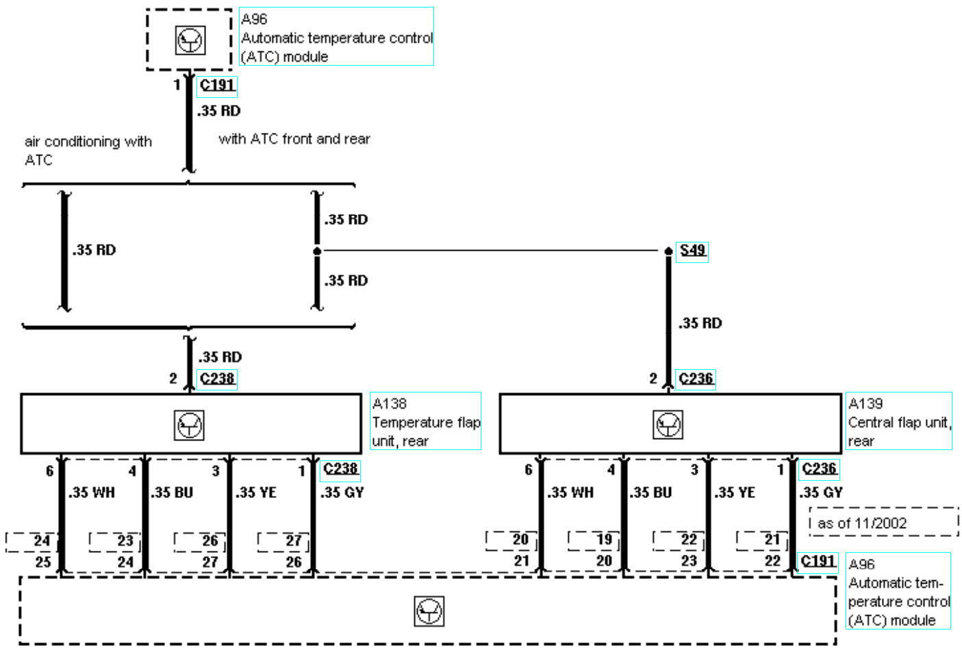
412-03A-00-024, Air Conditioning, Air conditioning with ATC module, 2,0i/2,3i DOHC, before 09/2000
